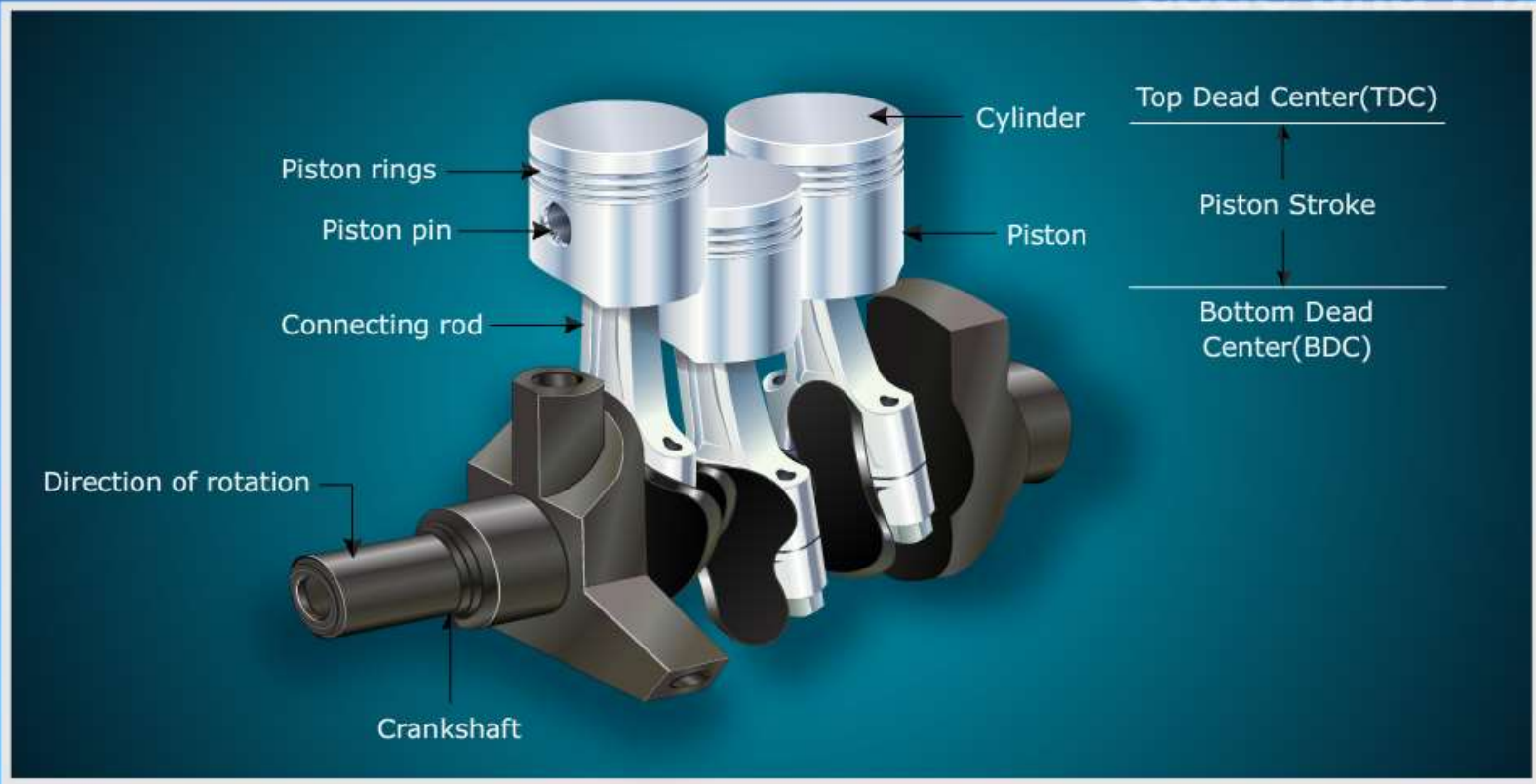
Rod/Piston Assembly from Cummins Diesel Engine
